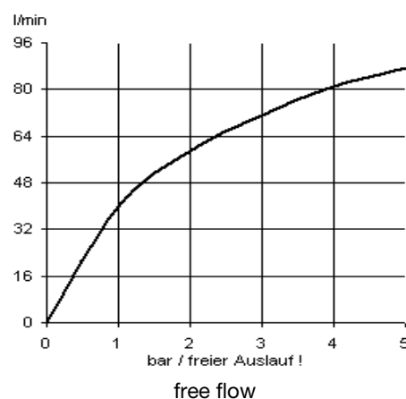
Flow rate diagram
