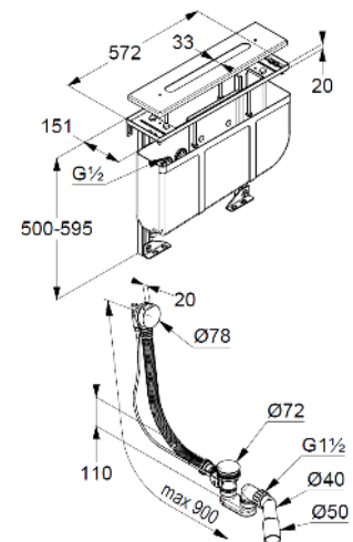
Dimensional drawing
